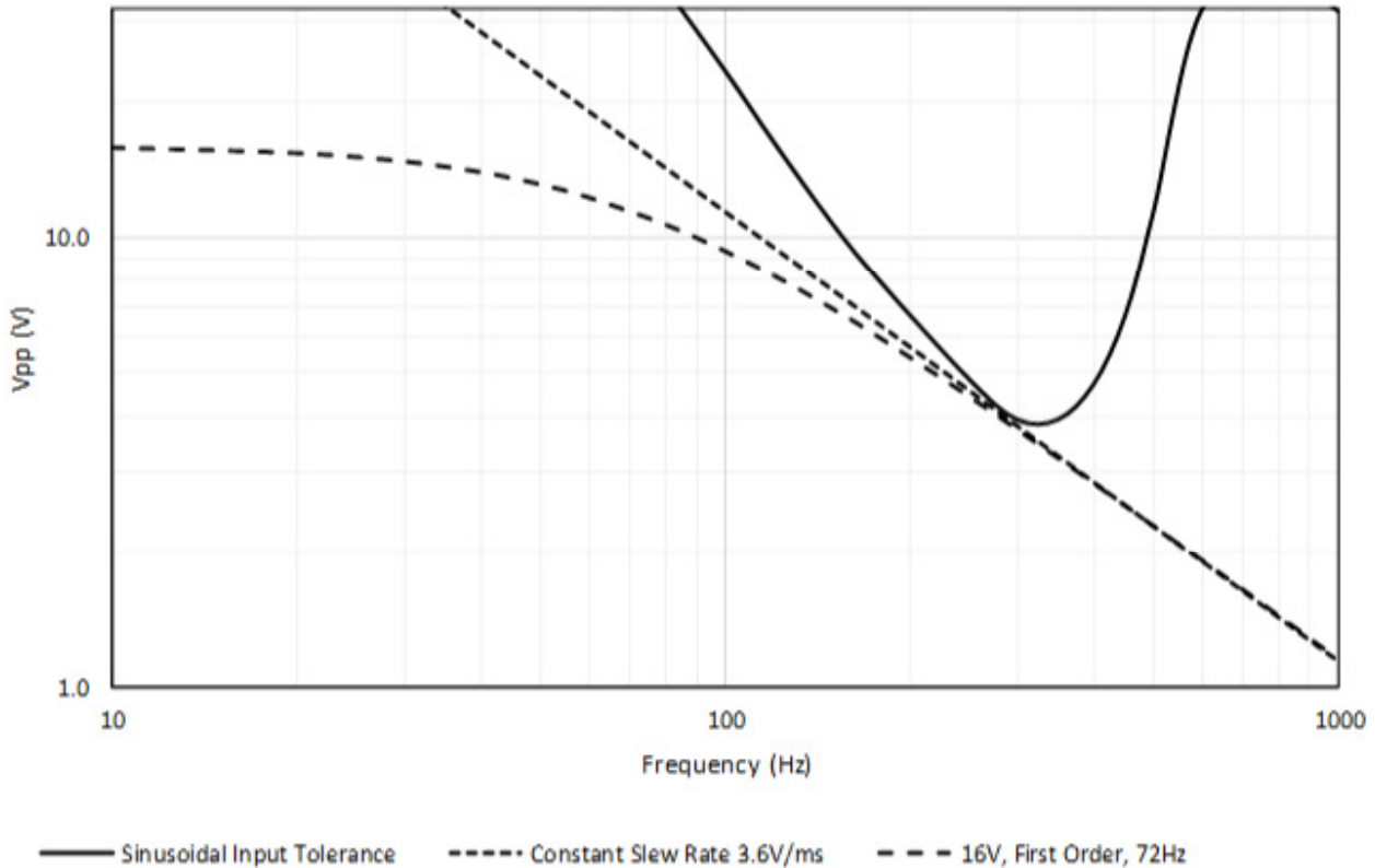
Figure 30 - Digital Input Slew Tolerance
