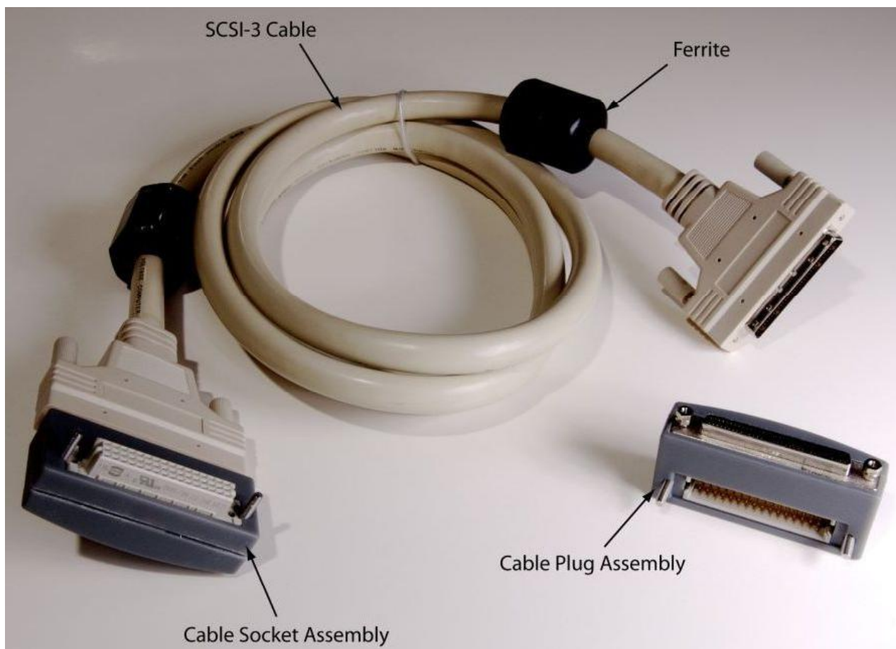
Figure 29 - Expansion Cable
